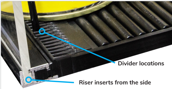
80mm High 4mm Powder-Coated Steel Wire 50, 70, 80, 110, 120mm High 3mm Stainless Steel Wire Dividers
